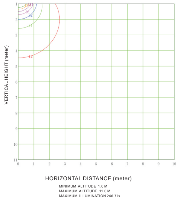
VERTICAL EQUILUMINOUS CURVE
